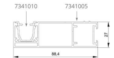
Single roller guide for ZF-A as standard.
